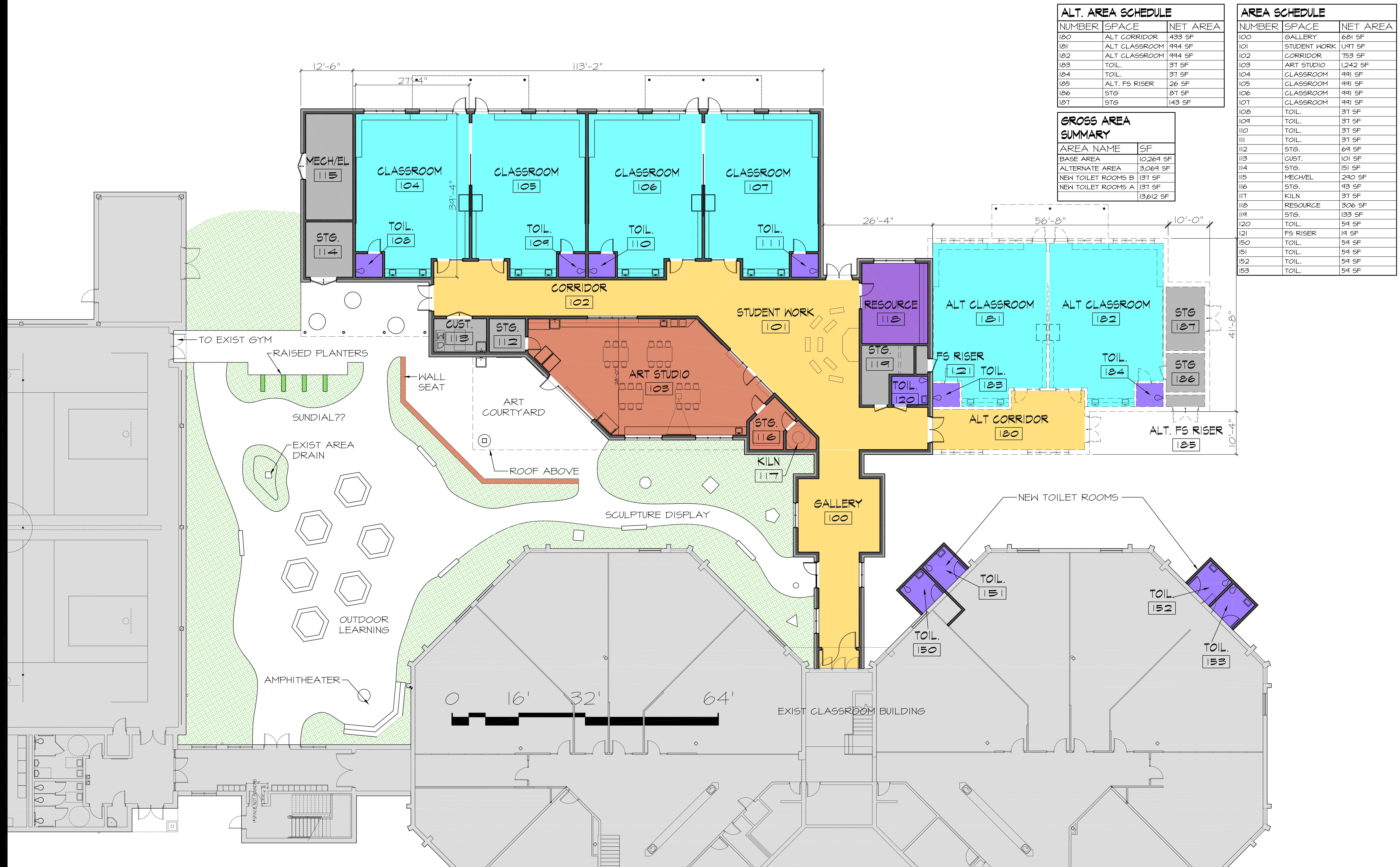
SK-01 PRELIMINARY LOWER LEVEL FLOOR PLAN C GREER ELEMENTARY SCHOOL ALBEMARLE COUNTY, VIRGINIA
